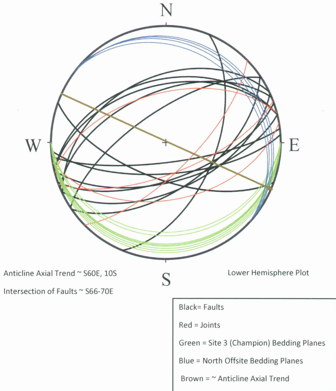
Figure 11. Stereo plot of geologic-structural elements of faults, joints and bedding planes at Proposed Yucca-Argyle Apartments.
