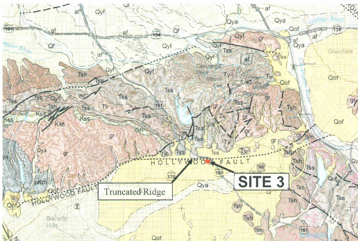
Figure 2: Geologic map of the area. Scale ~1:100,000. (California Geological Survey, Quaternary Geology Map of the Los Angeles 30x60 Quadrangle).
