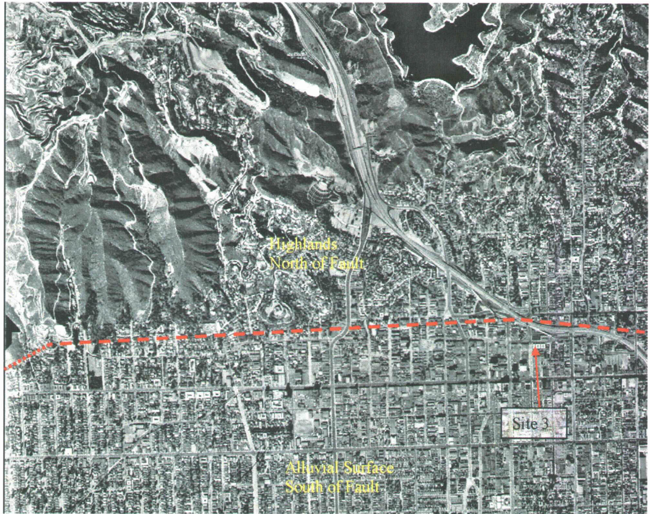
Figure 8: Approximate linear expression of the truncated ridges (red dashed line) based on aerial photo analysis. See Figure 6 for other geomorphic details. Scale unknown. (Continental Aerial Photo, 10-27-54).
